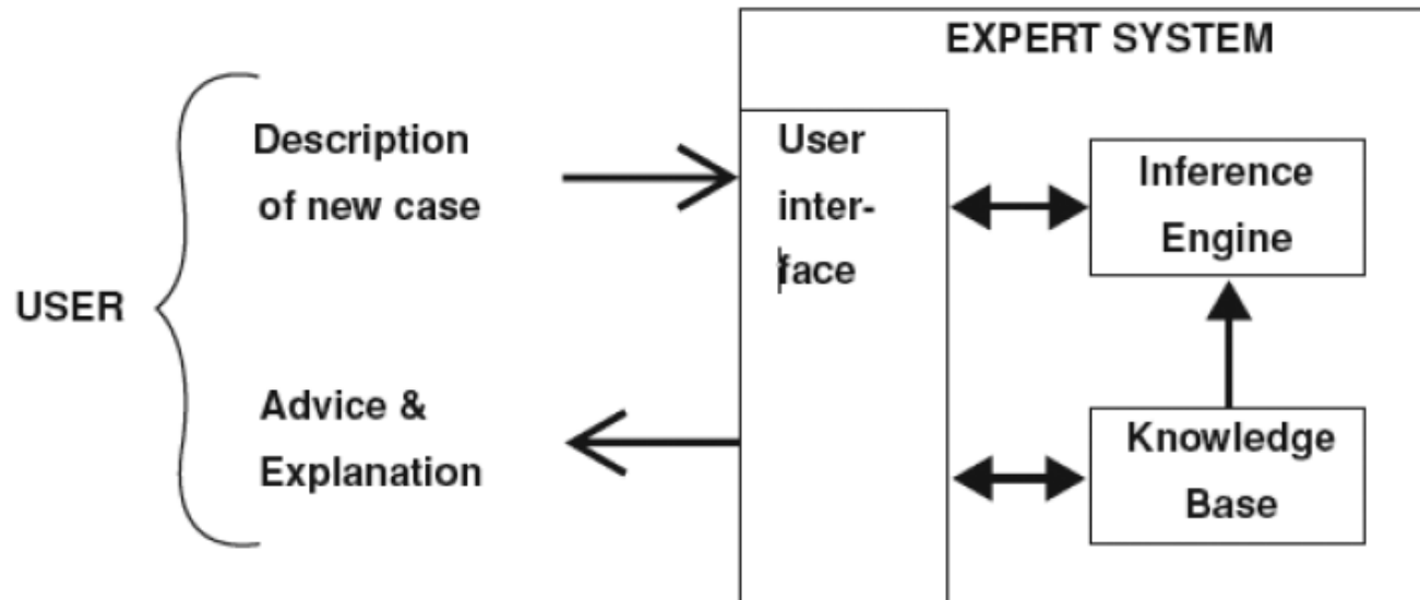
The structure of a MYCIN-style expert system
